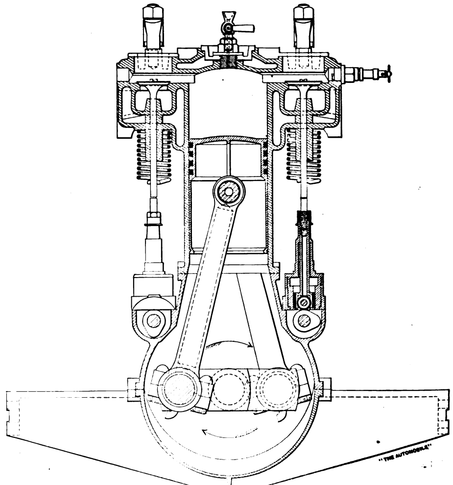
VERTICAL TRANSVERSE SECTION OF ONE OF THE CYLINDERS.
